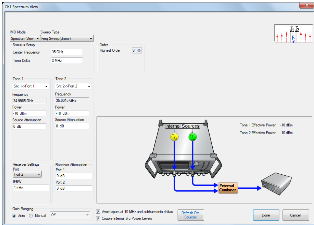
Figure 20-7. IMDView™ Configuration Dialog – SpectrumView Frequency Sweep (Linear)
