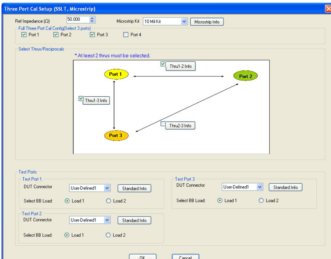
Figure 10-51. THREE PORT CAL SETUP (SSLT, MICROSTRIP) Dialog Box
