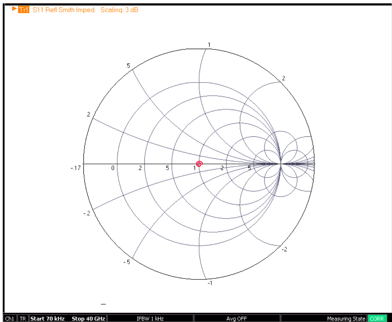
Figure 26-16. Compressed Smith Chart Example: 3 dB
