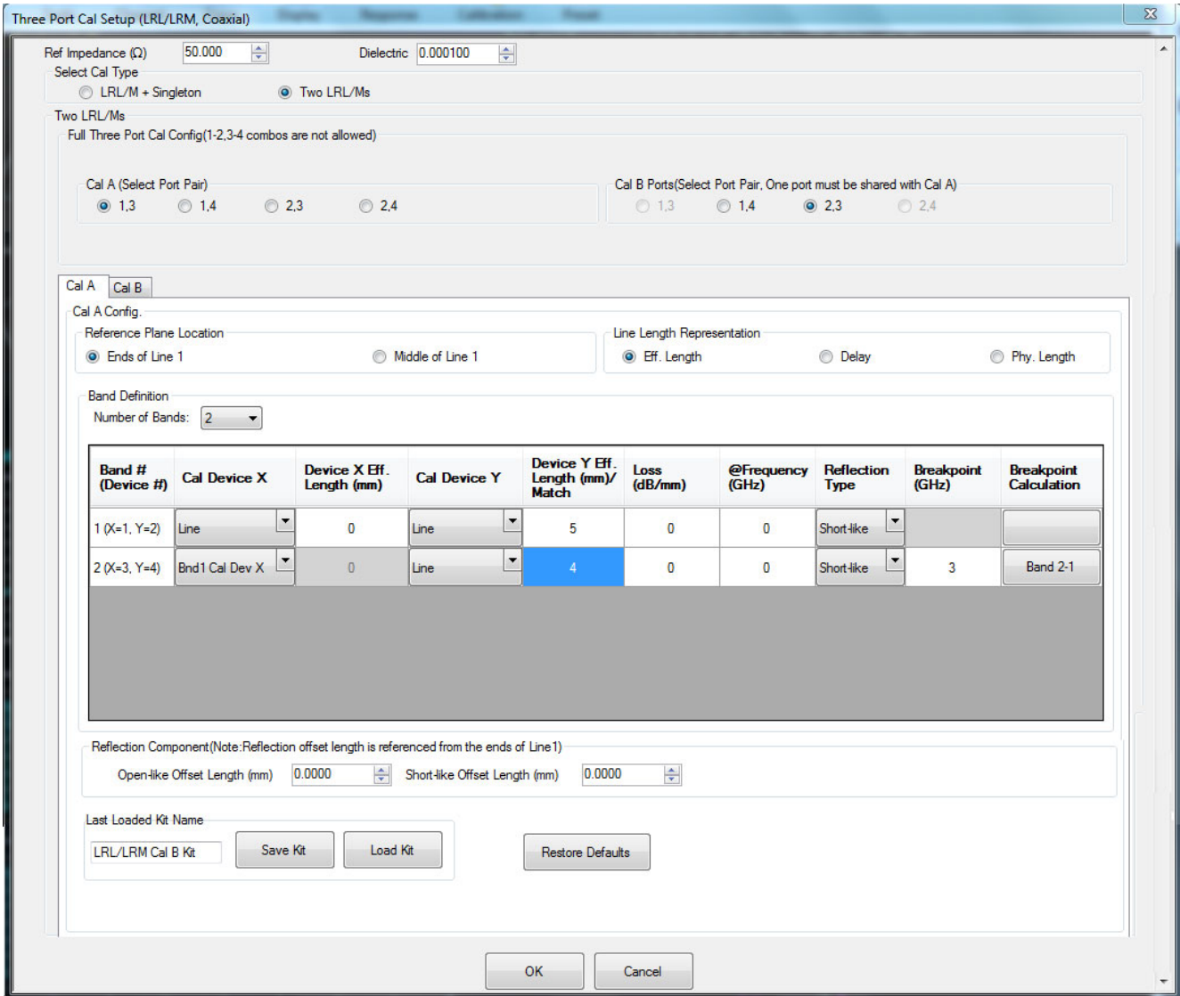
Figure 10-53. THREE PORT CAL SETUP (LRL/LRM, COAXIAL) Dialog Box - Cal A Tab
