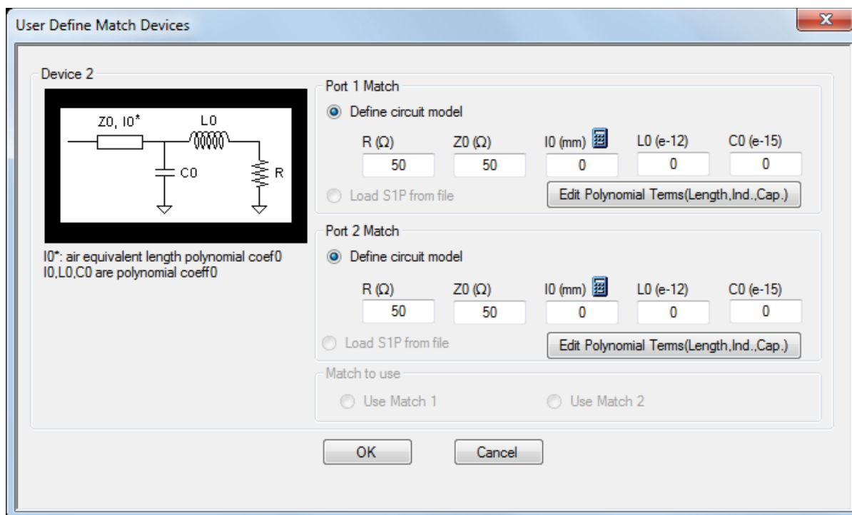
Figure 10-77. USER DEFINED MATCH DEVICES Dialog Box - LRL/LRM
