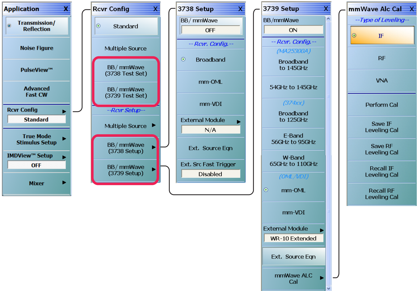
Figure 14-1. BB/mmWave Menus
