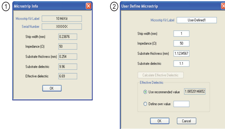
Figure 10-72. MICROSTRIP INFO and USER DEFINED MICROSTRIP Dialog Boxes
