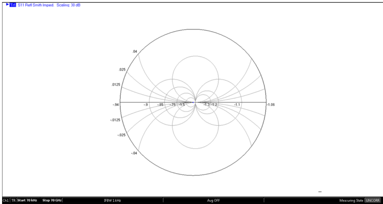
Figure 26-19. Compressed Smith Chart Example: 30 dB
