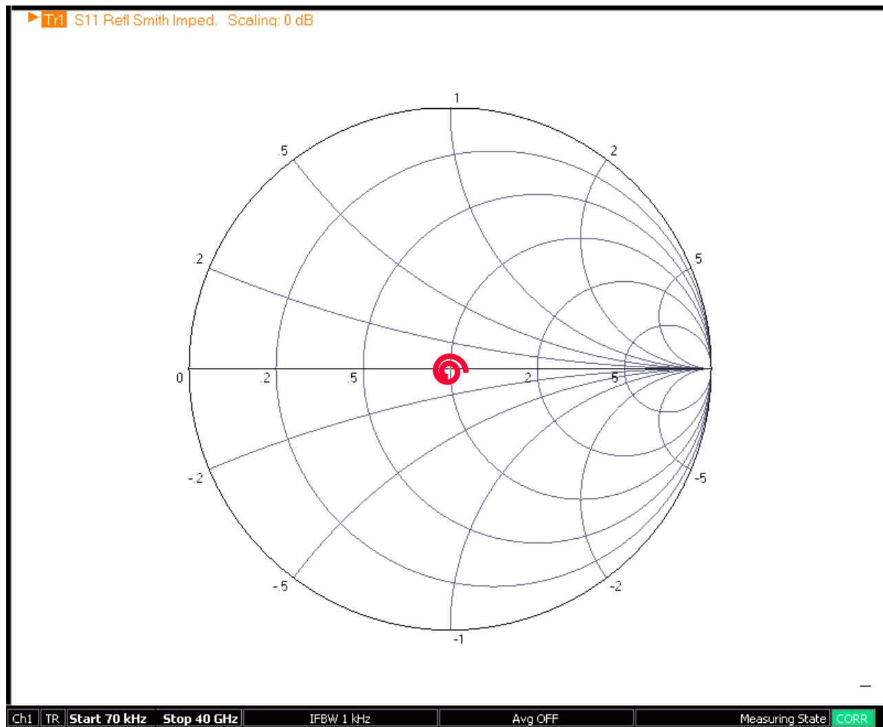
Figure 26-12. Smith Chart Impedance Display – Typical Results at 0 dB
