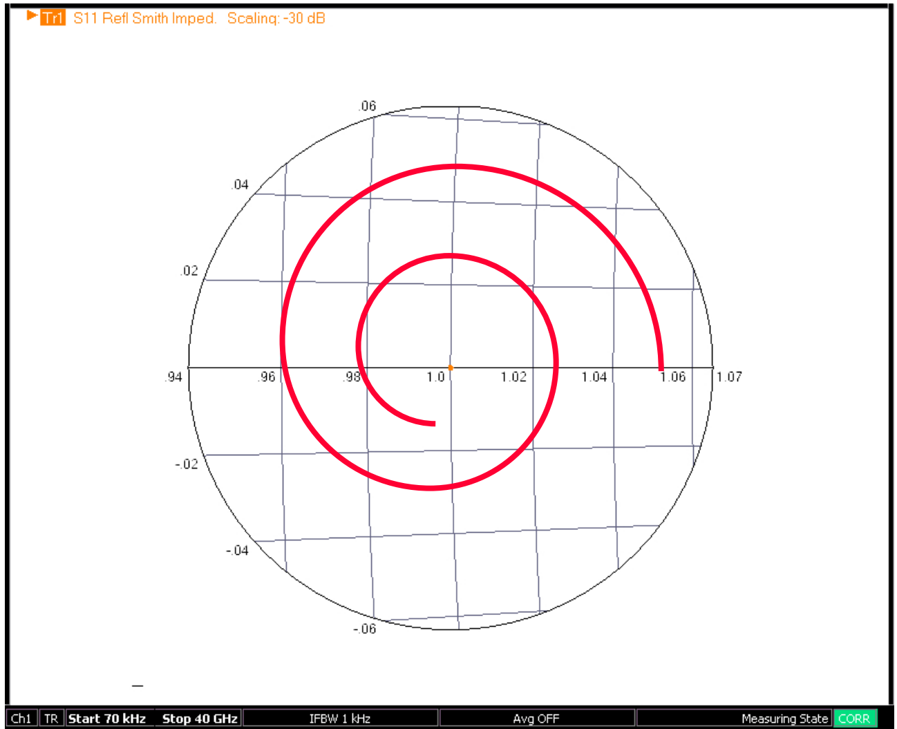
Figure 26-15. Smith Chart Impedance Display – Expanded to -30 dB
