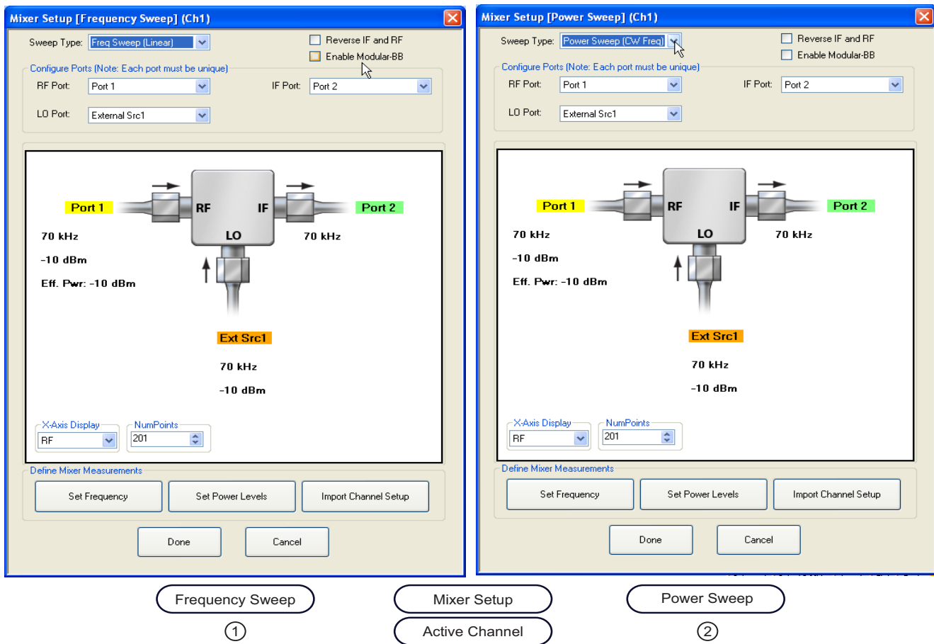
1. On left, MIXER SETUP (FREQUENCY SWEEP). 2. On right, MIXER SETUP (POWER SWEEP).
