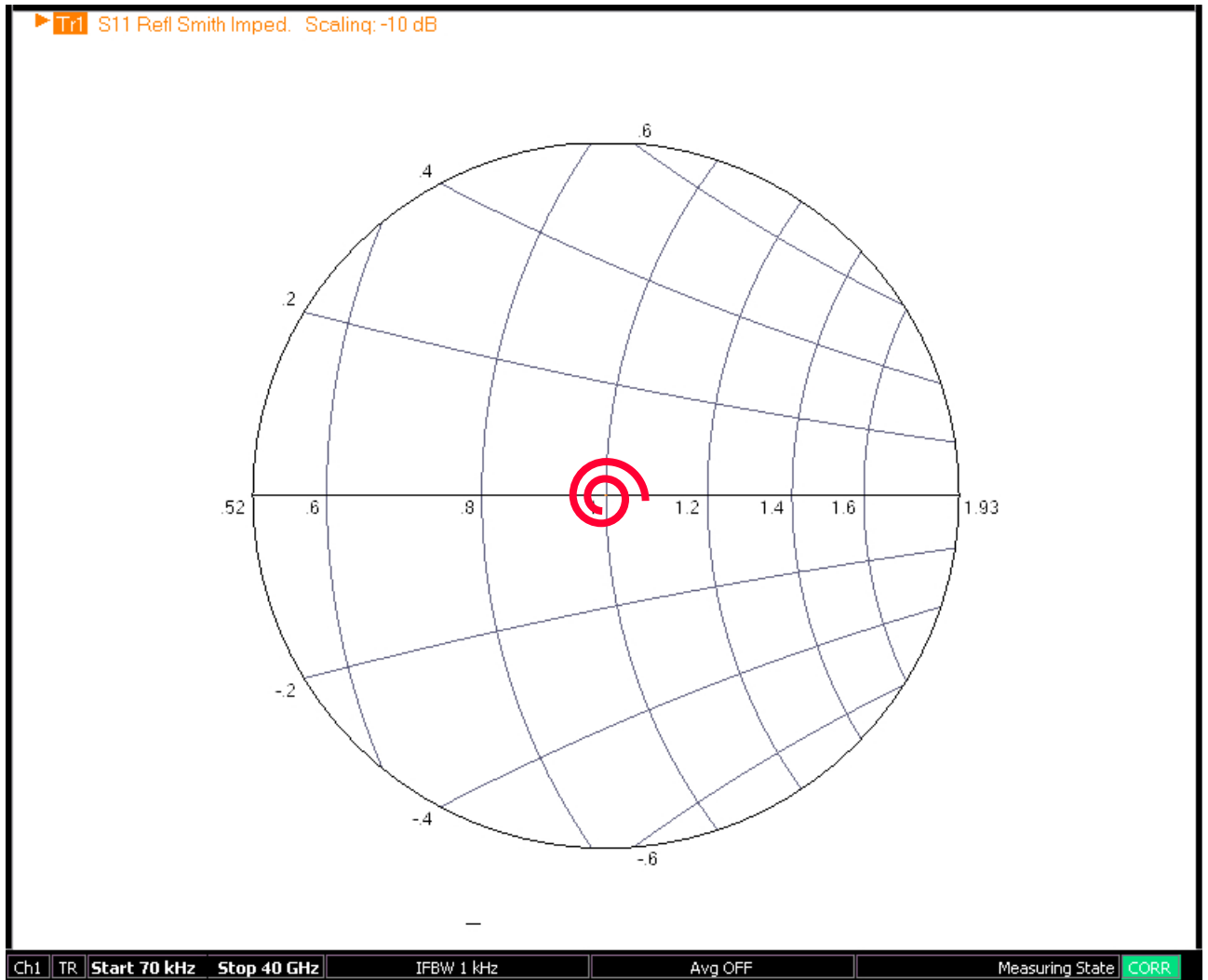
Figure 26-13. Smith Chart Impedance Display – Expanded to -10 dB
