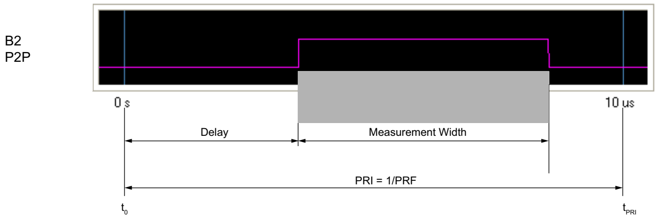
Figure 18-29. Pulse-to-Pulse Measurement
