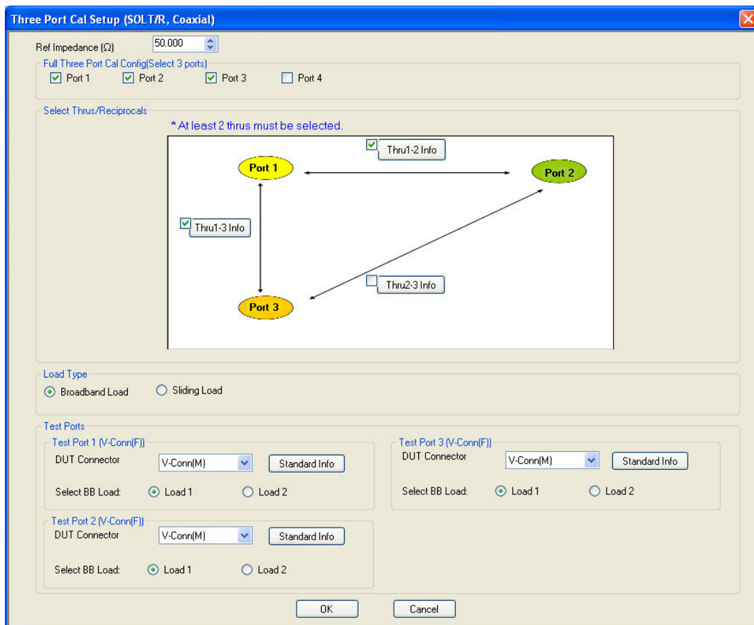
Figure 10-50. THREE PORT CAL SETUP (SOLT/R, COAXIAL) Dialog Box
