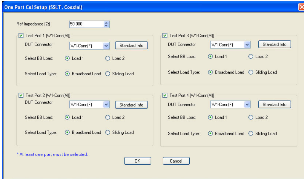
Figure 10-60. ONE PORT CAL SETUP (SSLT, COAXIAL) Dialog Box
