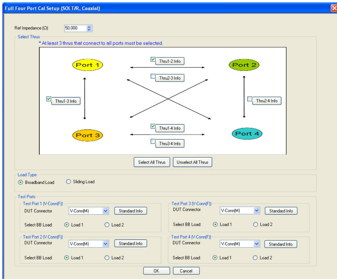
Figure 10-40. FULL FOUR PORT CAL SETUP (SOLT/R, COAXIAL) Dialog Box
