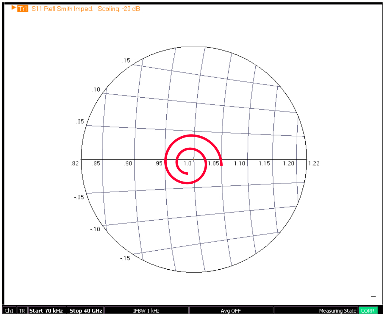
Figure 26-14. Smith Chart Impedance Display – Expanded to -20 dB
