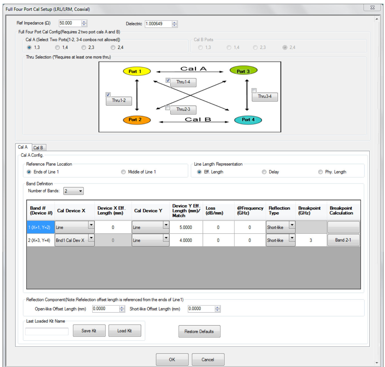
Figure 10-44. FOUR PORT CAL SETUP (LRL/LRM, COAXIAL) Dialog Box
