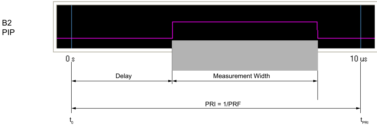
Figure 18-27. Point-in-Pulse Measurement
