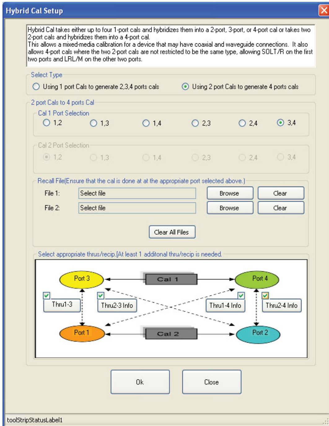
Figure 10-25. HYBRID CAL (CALIBRATION) Dialog Box – 4-Port VNAs
