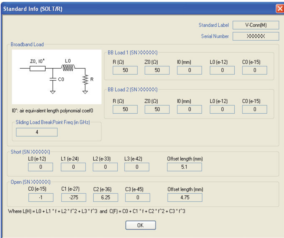
Figure 10-74. STANDARD INFO (SOLT/R) V-Conn (M)
