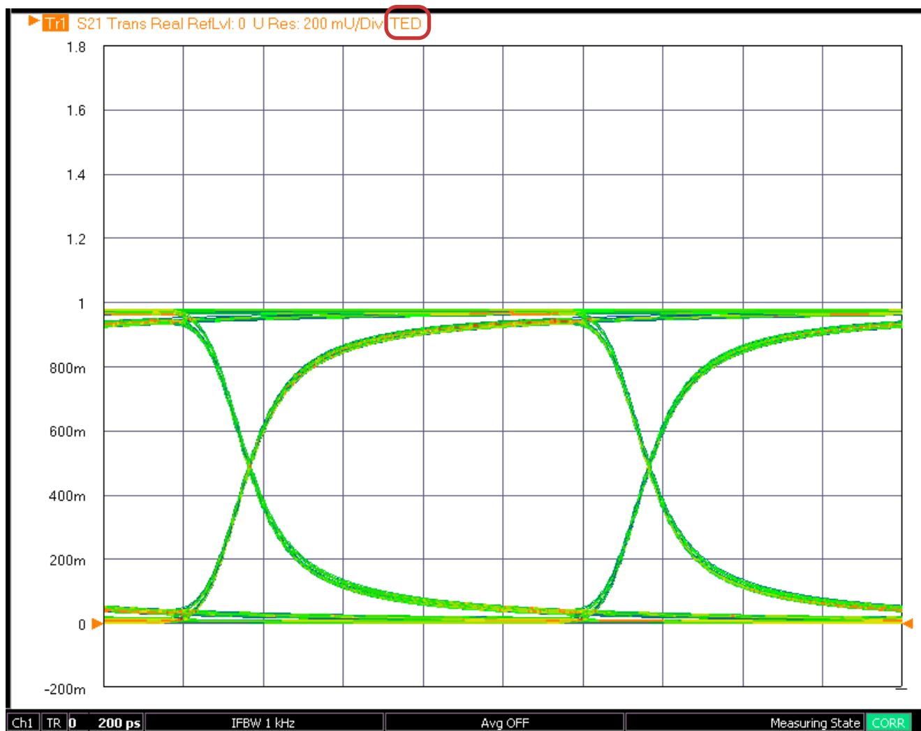
Figure 25-18. Time, Eye Diagram Display Example – Note that when in Time, Eye Diagram mode, the display trace annotation displays “TED”.
