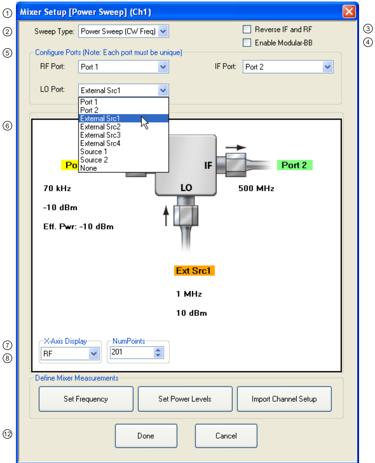
Figure 16-11. MIXER SETUP Dialog Box – Power Sweep – Control Locations (1 of 2)
