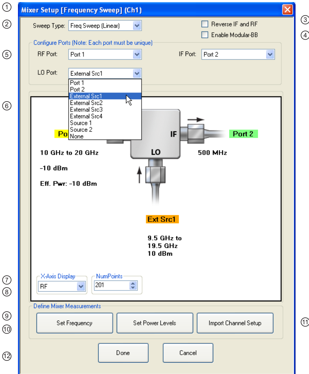
Figure 16-4. MIXER SETUP ACTIVE CHANNEL Dialog Box – Frequency Sweep – Control Locations (1 of 2)
