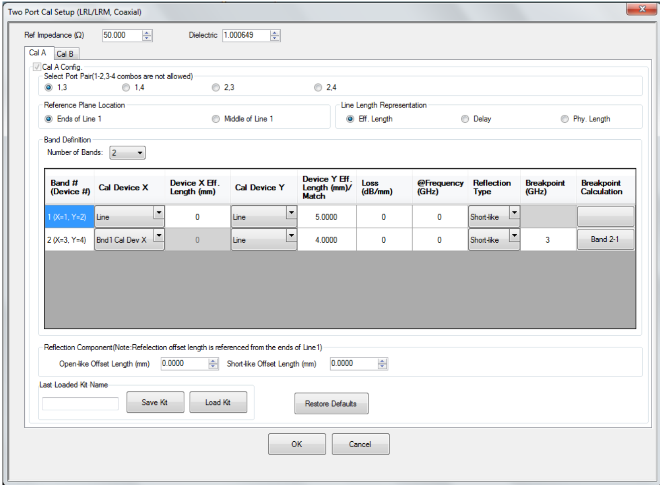
Figure 10-57. TWO PORT CAL SETUP (LRL/LRM, Coaxial) Dialog Box
